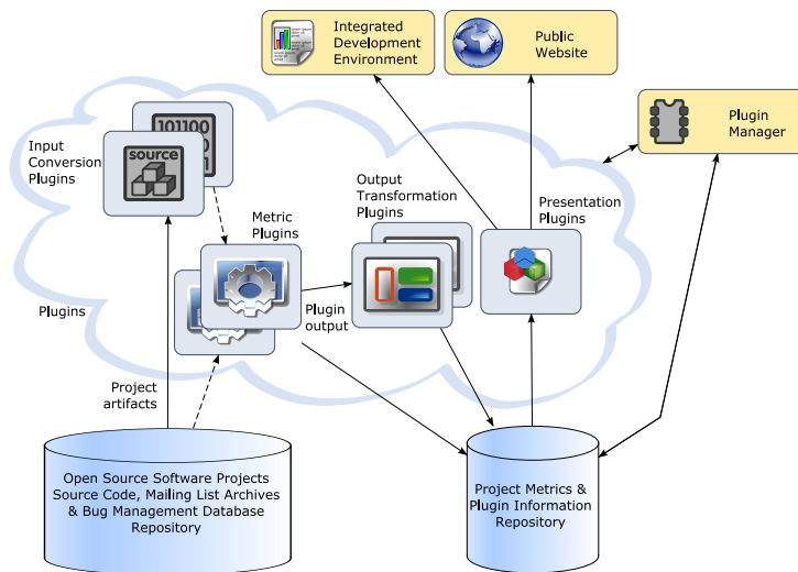
Fig. 1. SQO-OSS Platform Design
