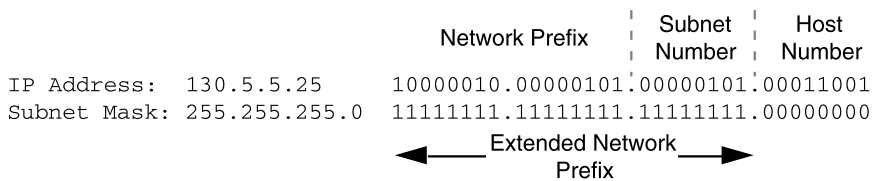
FIGURE 10. Subnet Mask
